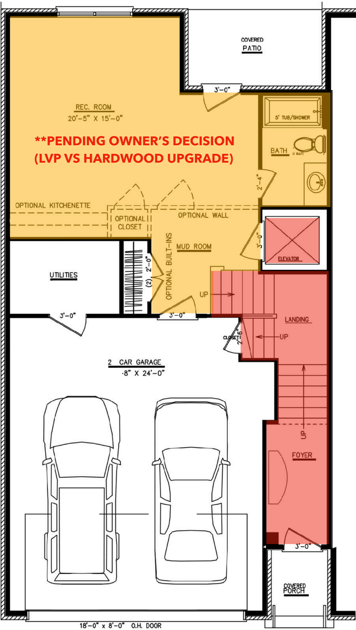
1st Floor
