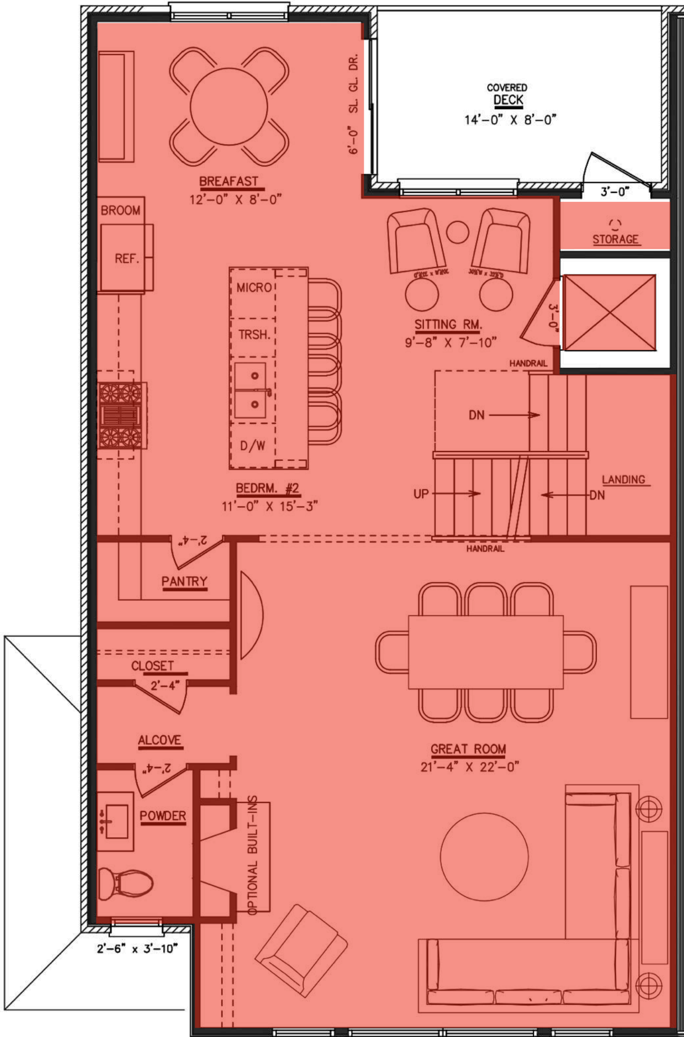
2nd Floor
