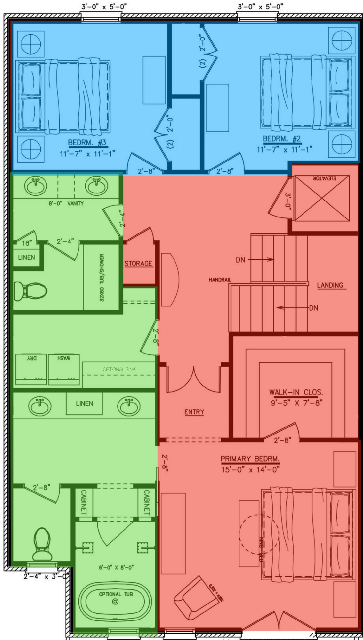
3rd Floor
